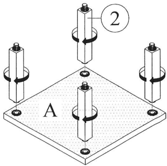
STEP 2 (5 TIER TOWER)
