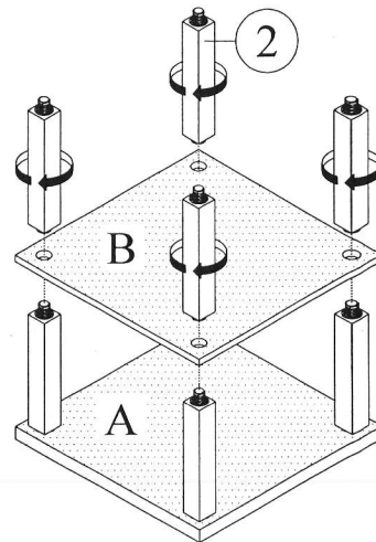
STEP 3 (5 TIER TOWER)
