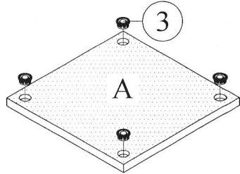
STEP 2 (5 TIER TOWER)
